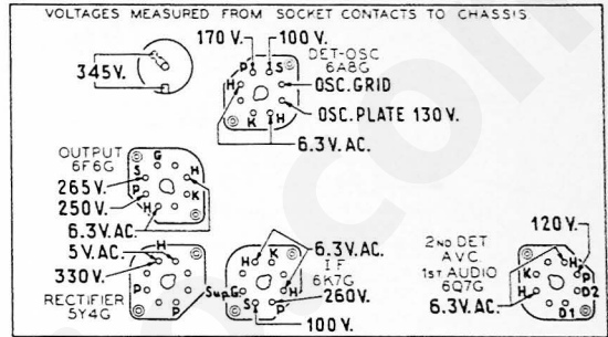
Fig. 1. Socket Voltages, Underside of Chassis
